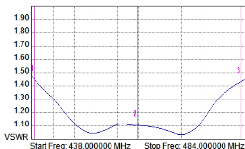
Diagrama Curva VSWR
